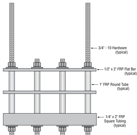
INTERMEDIATE HANGER / FLAT BAR-SQUARE TUBE BOTTOM
