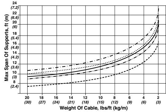
2" XW DIAMETER
