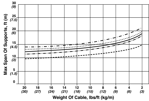
3" XW DIAMETER
