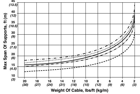
6" MW DIAMETER
