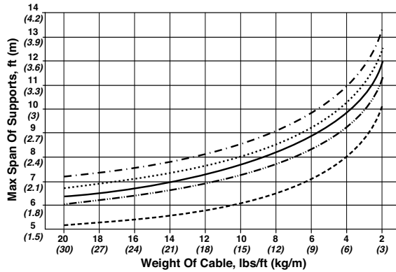
2" SW DIAMETER
